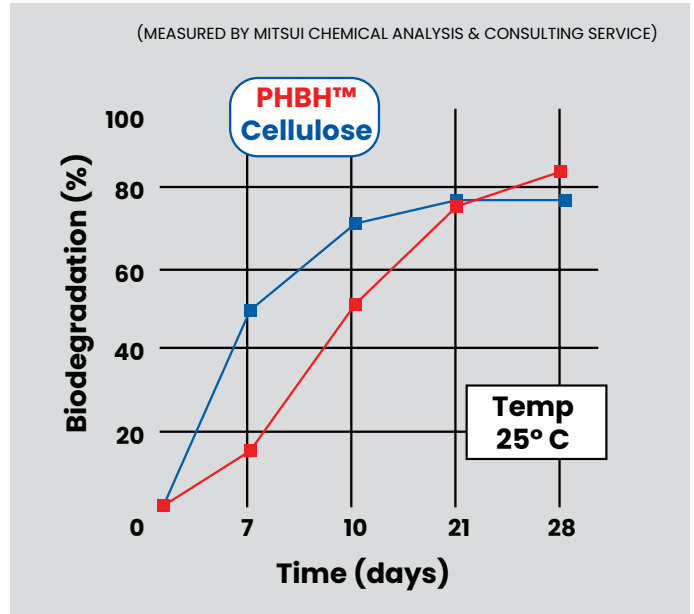
ISO14851 (ACTIVATED SLUDGE) TESTS WERE PERFORMED ON RESIN POWDER
