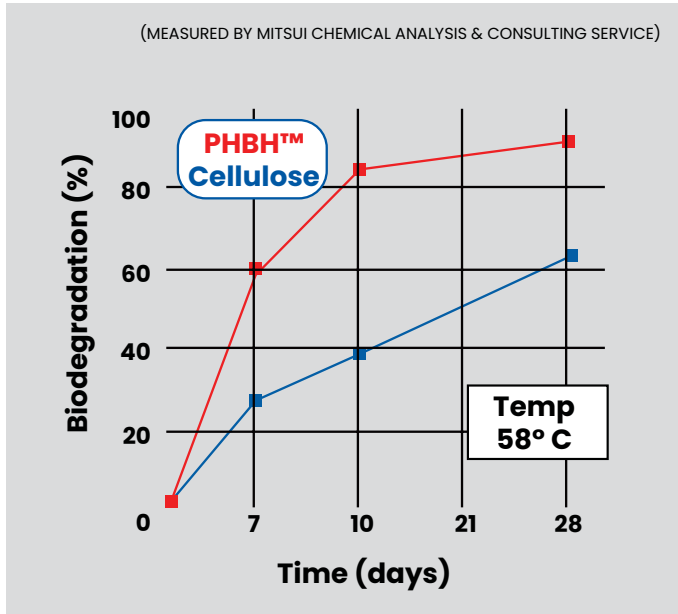
ISO14855 (COMPOST) TESTS WERE PERFORMED ON RESIN POWDER
